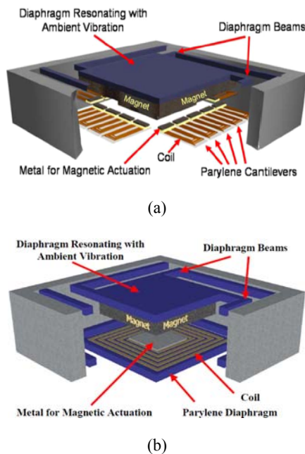
Fig. 4. Model of generator: (a) first generator module, (b) second generator module.
