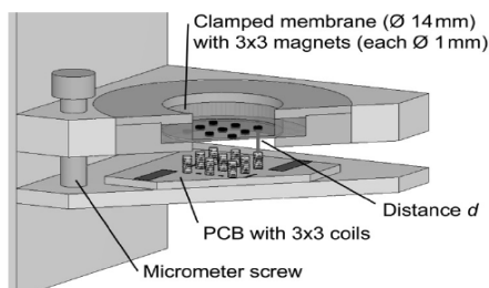
Fig. 7. Schematic view of generator.
