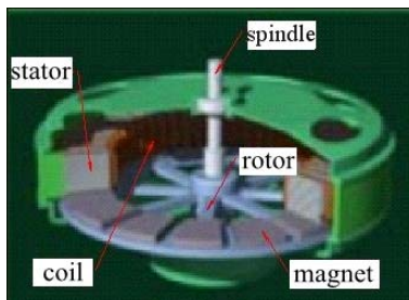
Fig. 1. Diagram of rotational magnetic generator.
