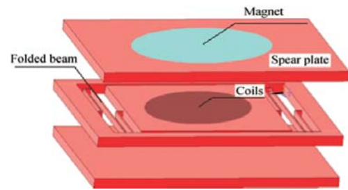
Fig. 8. Schematic structure.
