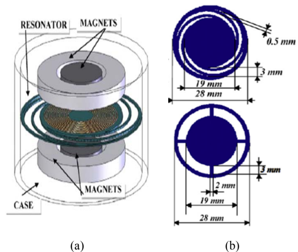
Fig. 3. (a) Generator structure; (b) two resonator structures.
