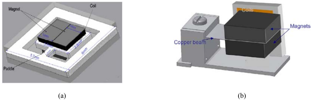
Fig. 9. Generators: (a) Prototypes A/B; (b) prototype C.
