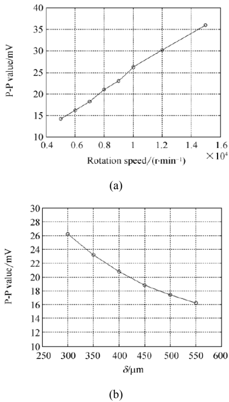
Fig. 2. (a) Induced voltage changes with rotational speed, (b) Induced voltage changes with air gap.
