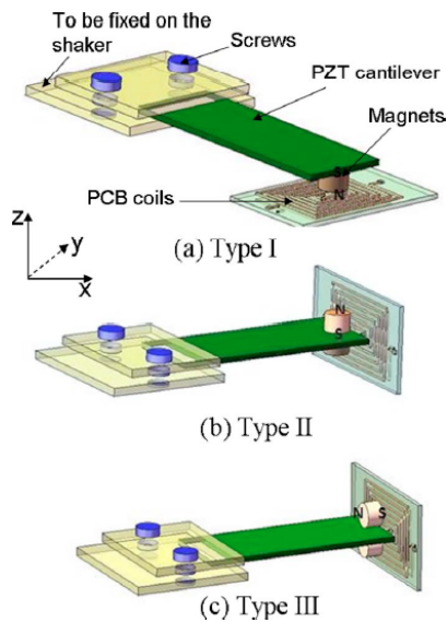
Fig. 11. Hybrid generator (a) type I, (b) type II, (c) type III.
