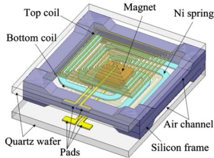
Fig. 6. Generator structure with air channel.
