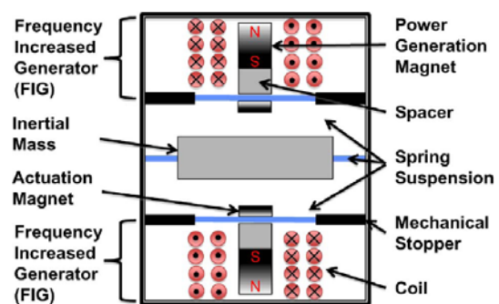
Fig. 5. PFIG structure.
